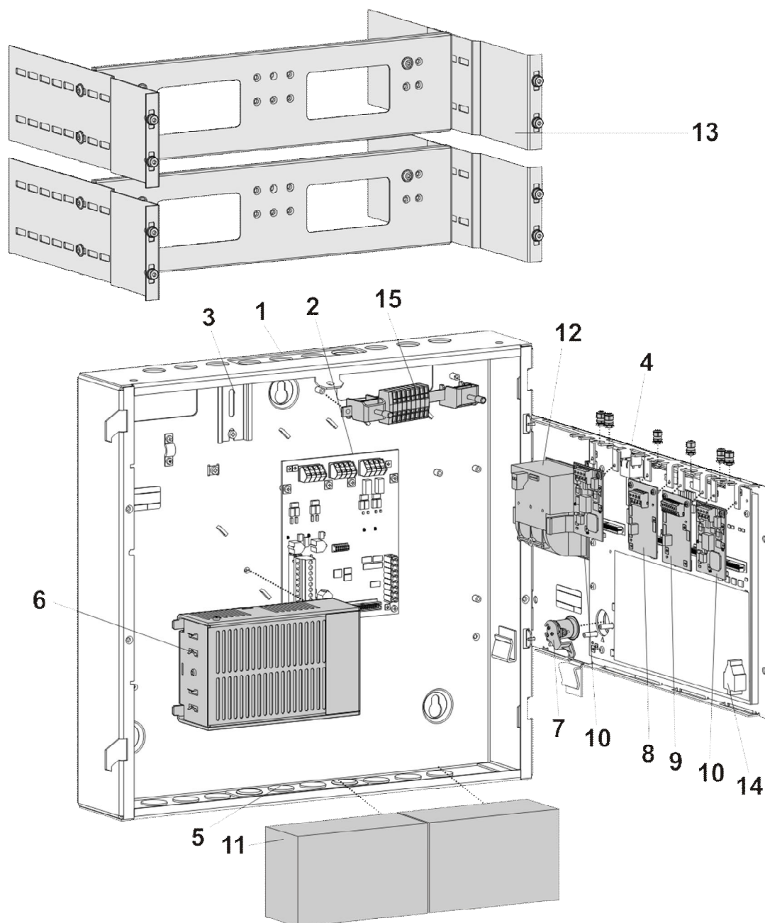
Layout of FT724
